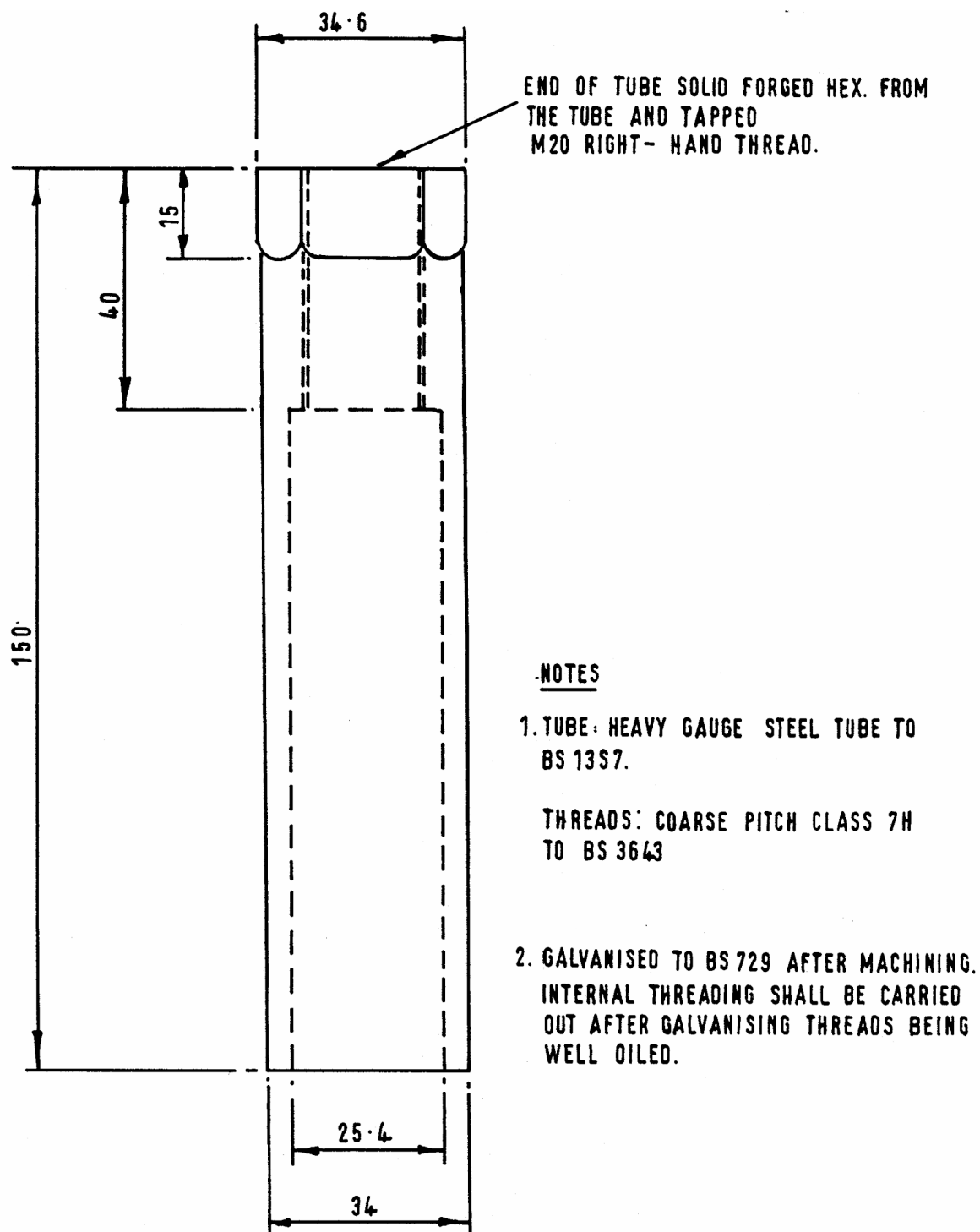
Figure 53: Temporary earth attachment nut (ESI Drawing No. 439554) (132 kV Lines to ESI Standard 43-50)
